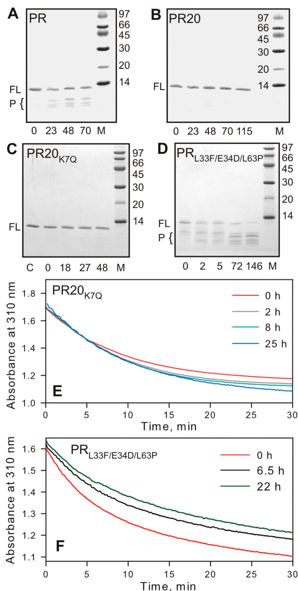
Figure 2. Time course of autoproteolysis of (A) PR, (B) PR20, (C) PR20 K7Q and (D) PR L33F/E34D/L63P at room temperature in 50 mM sodium acetate buffer, pH 5. Proteins were folded from 12 mM HCl by a quench protocol, as previously described, 25 to give a final concentration of 13 \mu M (as dimer) in 50 mM acetate, pH 5. Samples were withdrawn at the indicated times (in hours), mixed with gel loading buffer and analyzed by sodium dodecyl sulfate polyacrylamide gel electrophoresis (SDS-PAGE) (20% homogeneous PhastGel, GE Healthcare). FL and P designate full length protease and products of autoproteolysis, respectively. M denotes molecular weight markers in kDa. Numbers below the gels denote hours of incubation at room temperature. (C) and (E) show that PR20 bearing the wild-type residue in position 7 (K7Q) is equally resistant to autoproteolysis as PR20. Sample PR20 K7Q prior to initiating the assay is shown in lane C (panel C). (E and F) Time dependent decrease in protease mediated hydrolysis of substrate IV assayed at the indicated times at a final enzyme concentration of 440 nM for PR20 K7Q and 330 nM PR L33F/E34D/L63P and final substrate concentration 380 \mu M, 28 °C. PR L33F/E34D/L63P shows a significant decrease in catalytic activity with increasing time of incubation, consistent with appearance of products of autoproteolysis, unlike PR20 or PR20 K7Q (compare (B) and (C) with (D)). (D) and (F) demonstrate that mutations L33F and L63P are not responsible for the reduced rate of autoproteolysis seen with PR20 consistent with a rate comparable to wild-type PR.
