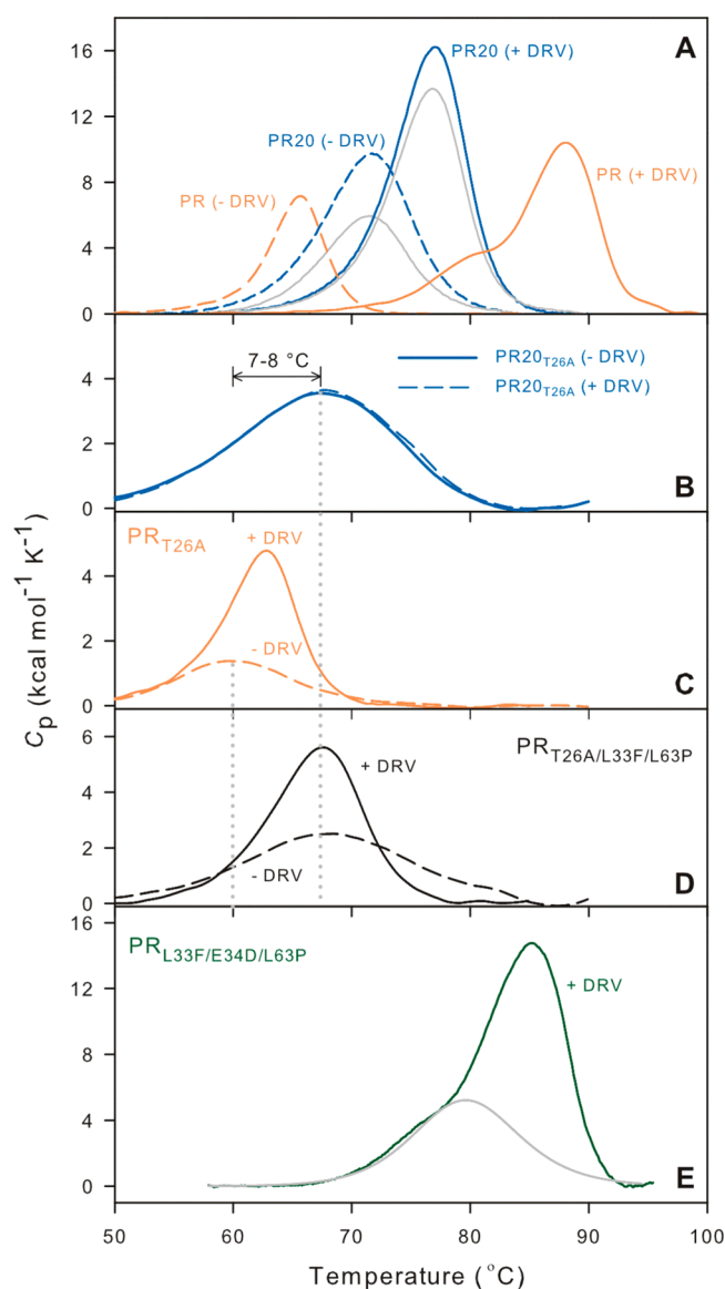
Figure 5. Differential scanning calorimetry of PR, PR20, and PR L33F/E34D/L63P dimers (A and E) and its corresponding monomers (B–D). Dashed and solid lines are thermal denaturation curves in the absence and presence of DRV, respectively. (A) Orange lines correspond to PR and blue to PR20. Traces shown in gray for PR20, obtained on a second scan of the DSC sample after completion of the initial scan, indicate partial reversibility of thermal melting in both the presence and absence of DRV. Data for PR, shown for comparison, are from. 21 Panels B–D show the effect of DRV on the thermal denaturation of PR20, PR, and PR L33F/L63P monomers bearing the T26A mutation. The absence of any effect of DRV on PR20 T26A (B) indicates that this monomer likely does not form a complex with DRV. (E) Thermal denaturation of PR L33F/E34D/L63P dimer as its DRV complex (green). The curve in gray represents deconvolution of a transition with T_m = 79.7 ^\circ\text{C} , analogous to that seen in the biphasic DSC plot for PR (panel A). For values of T_m and \Delta T_m derived from these plots, see Table 1A.
