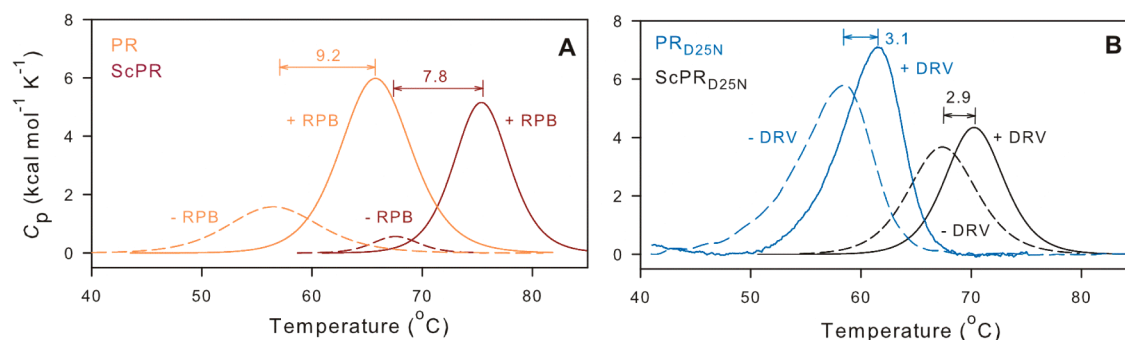
Figure 6. Effect of dimer stability on inhibitor binding and thermal denaturation of single-chain PR constructs ScPR (dark red) and ScPR D25N (black) in comparison with PR (orange) and PR D25N (blue) homodimers. Dashed and solid lines designate scans without inhibitor and with ~2-fold molar excess of inhibitor RPB or DRV relative to the respective proteases (as dimers). \Delta T_m values shown for each pair of traces show the increase in T_m of each protein upon inhibitor binding. For experimental details, see the Materials and Methods section. Actual T_m values are given in Table 1B.
