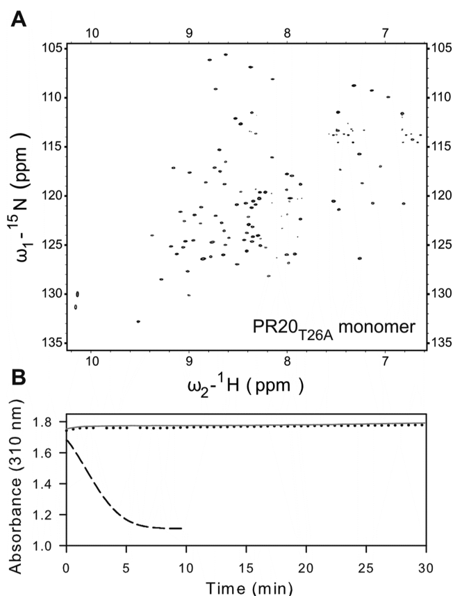
Figure 4. (A) 600 MHz ^1\text{H} – ^{15}\text{N} TROSY-HSQC spectrum of freshly prepared uniformly ^{15}\text{N} - and ^{13}\text{C} -labeled PR20 T26A (100 \mu\text{M} as monomer) in 20 mM sodium phosphate buffer, pH 5.8, 20 ^\circ\text{C} . A spectrum acquired using a 4-fold diluted sample (not shown) clearly superimposes on the one shown, indicating that no changes occurred in the monomer–dimer or tertiary fold status, and that the protein is all monomeric in conjunction with data shown in (B). (B) Activity assays with 360 \mu\text{M} substrate IV in 50 mM sodium acetate buffer, pH 5, containing 250 mM NaCl. Dotted black and solid gray lines are for 1 and 5 \mu\text{M} PR20 T26A (as dimer), respectively. For comparison, the dashed line is for 300 nM active PR dimer shows depletion of substrate within 5 min.
