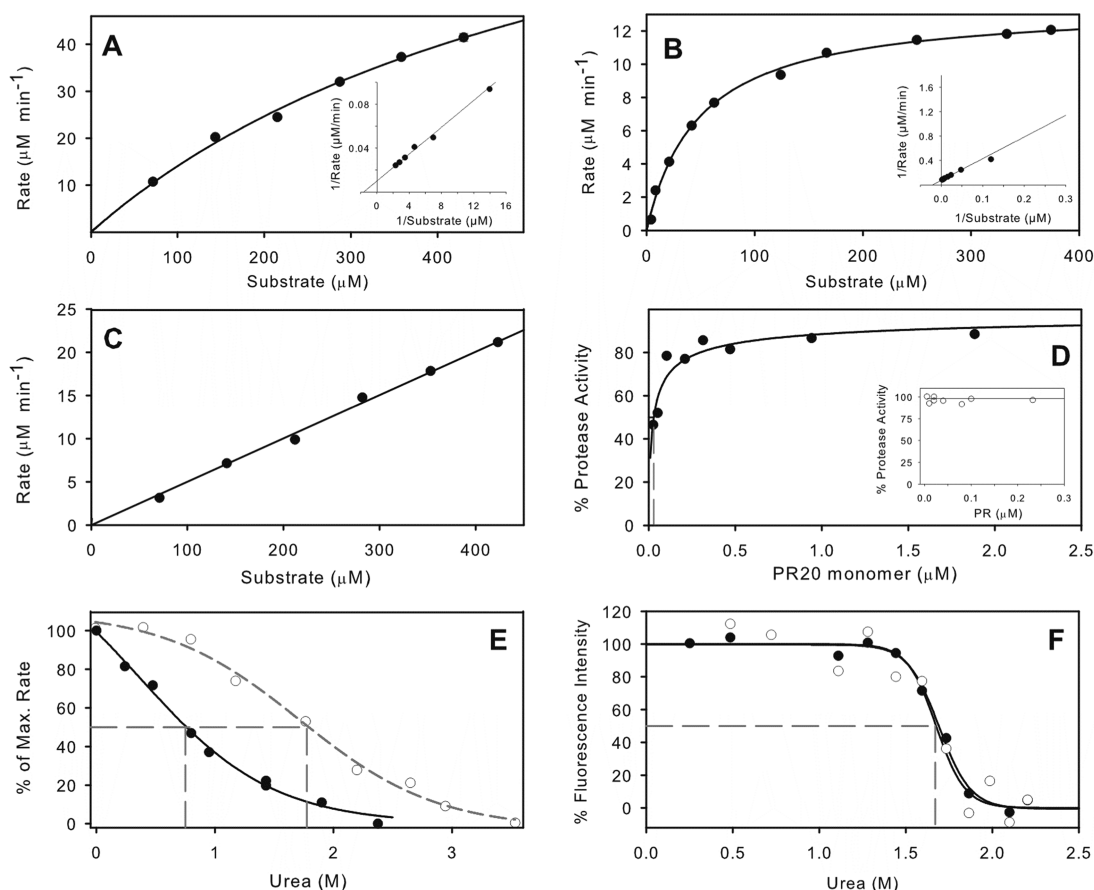
Figure 3. Kinetic properties of PR20 and comparison with PR. Michaelis–Menten kinetics for hydrolysis of substrate IV by 0.5 \mu\text{M} PR20 in 50 mM sodium acetate buffer, pH 5, containing 250 mM sodium chloride (A), and its hydrolysis under the same conditions 31 catalyzed by 80 nM PR. (B) Kinetic parameters for PR20 are k_{\text{cat}} \geq 196 \text{ min}^{-1} and K_{\text{m}} \geq 533 \mu\text{M} . For PR, k_{\text{cat}} = 174 \pm 3 \text{ min}^{-1} and K_{\text{m}} = 48.2 \pm 3.1 \mu\text{M} . Solid lines are based on curve fitting of the Michaelis–Menten equation to the data. Lineweaver–Burke plots are shown as insets. (C) The linear dependence of reaction rate for PR20 hydrolysis on substrate concentration, resulting from an increased K_{\text{m}} in the presence of 0.8 M urea under the same conditions as in (A). (D) Dependence of catalytic activity on the concentration of PR20 in the same buffer gives a K_{\text{d}} of 29 \pm 10 \text{ nM} (dashed gray line). For comparison, the inset shows that the K_{\text{d}} for PR is <5 \text{ nM} under similar conditions. 20 (E) Effect of increasing urea concentration on hydrolysis of substrate IV by PR20 (●) and by PR (○). (F) Effect of urea concentration on the intrinsic fluorescence of PR20 in 50 mM sodium acetate buffer, pH 5; data in the absence of inhibitor (●) and in the presence of 2 \mu\text{M} DRV (○). The urea concentrations at which 50% of the maximum effect ( \text{UC}_{50} ) is observed are indicated by dashed gray lines in (E) and (F).
